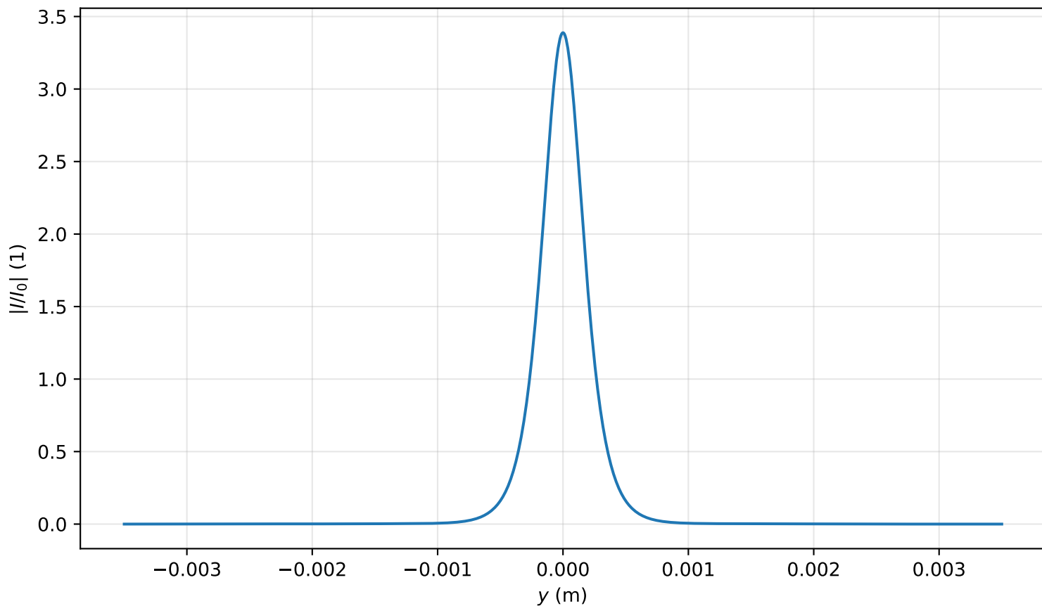
Intensity profile I(x = 0, y, z = 3.981)/I_0 , P_{in}=1.0P_{cr} , artificial time
